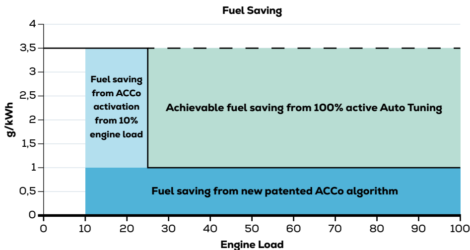
Figure 1: Fuel saving
