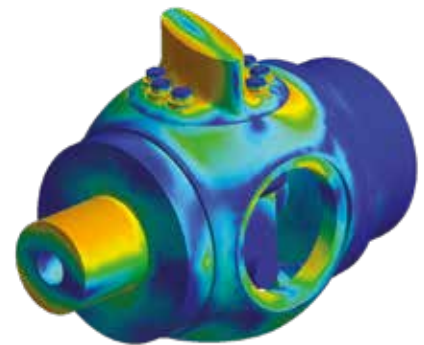
FEM analysis: propeller hub assembly subjected to simulated shock from underwater explosion
