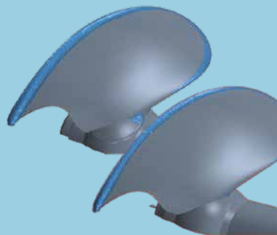
High blade loading simulation – reduced root cavitation below
