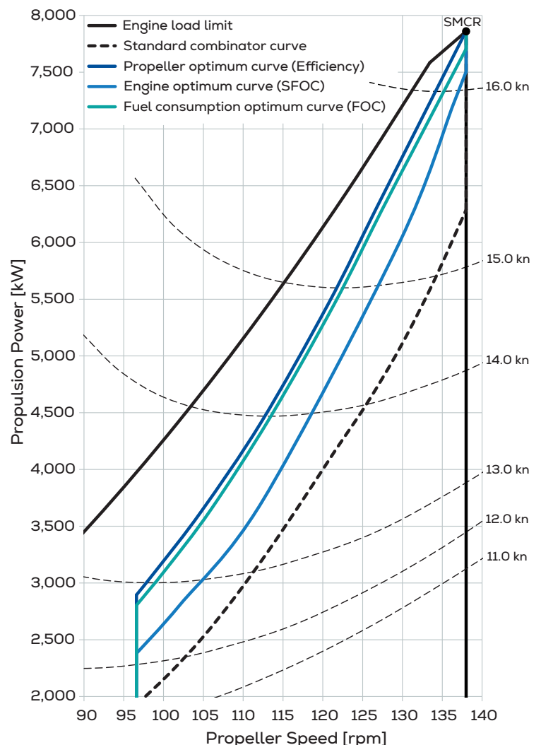
Fig. 27: Optimum propeller (Efficiency), engine (SFOC), and EcoOptimizer (FOC) curves
