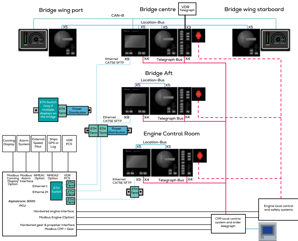
Fig. 45: Alphasatronic 3000 networks architecture
