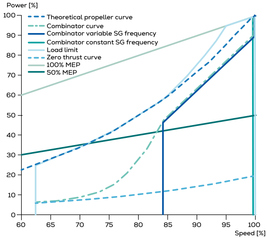
Fig. 40: Simple load diagram
