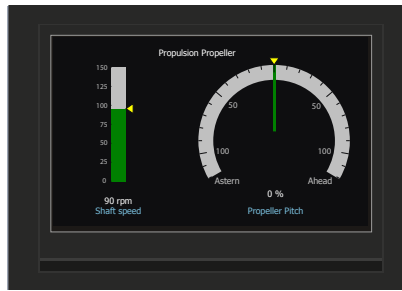
Fig. 28: Panama instrument – Propeller Indicator Panel – PIP standard indoor version
