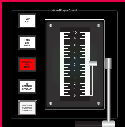
Fig. 36: Two-stroke Engine Handle Panel – EHP
